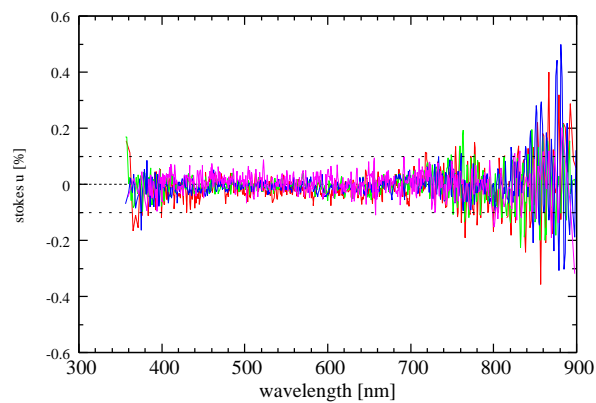
stokes u [%]
