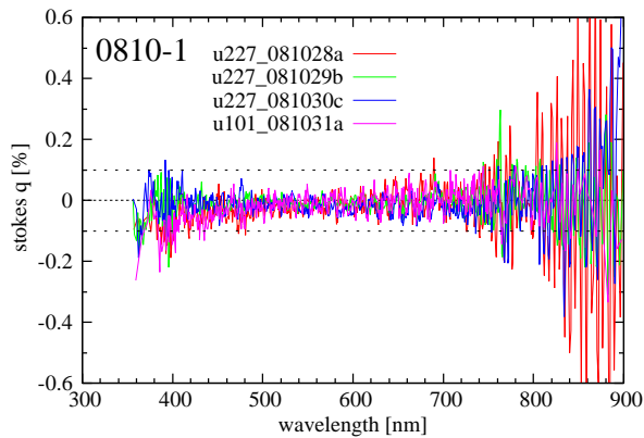
stokes q [%]
